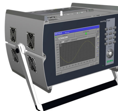
MT551 Current and voltage source 120 A / 500 V
